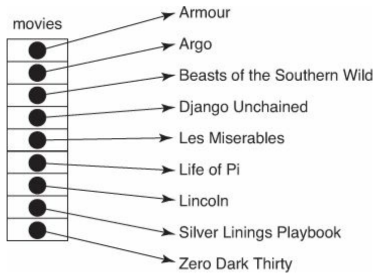
FIGURE 25.2 The movies array contains pointers to strings.
