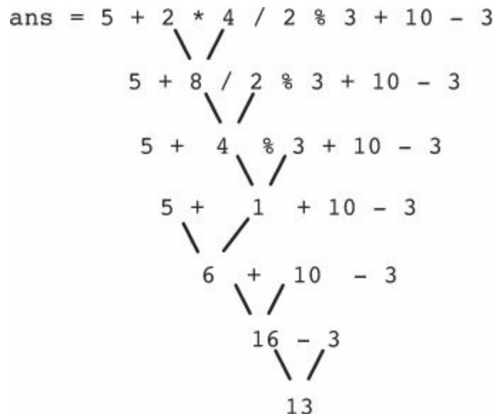
FIGURE 9.1 Solving the expression the way C would.
