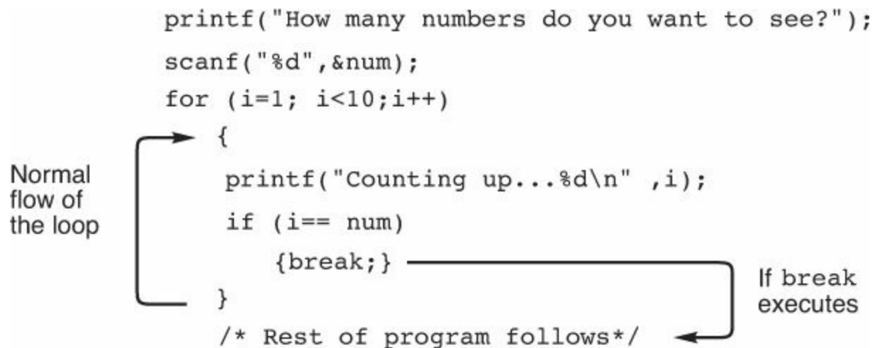
FIGURE 16.1 break terminates a loop earlier than usual.
