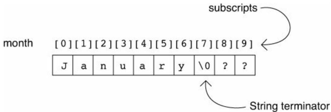
FIGURE 6.2 Defining and initializing an array named month that holds string data.
